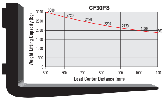
Lifting Capacities
