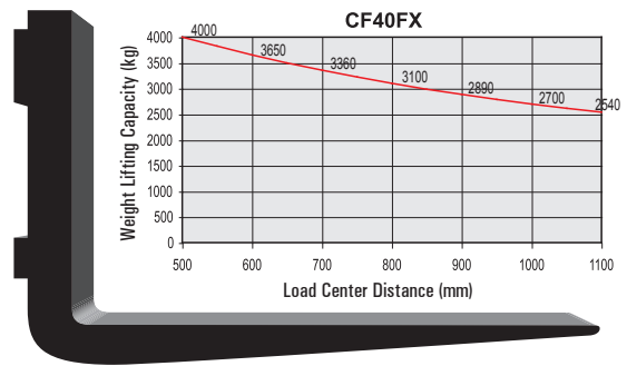
Lifting Capacities
